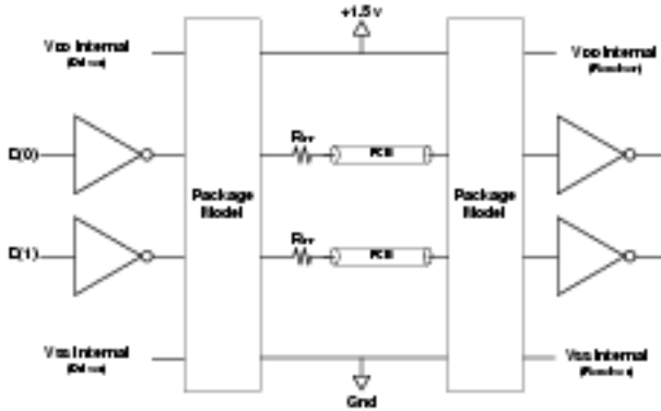
Fig. 1. Test Circuit Used to Analyze Bus Configuration (showing a 2:1:1 SPG Ratio)
