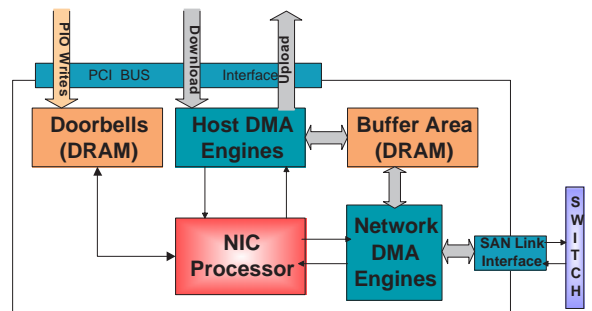
Fig. 2. A standard NIC Architecture
