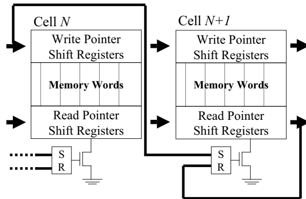
Fig. 4. Sleep Mode Buffer Architecture
