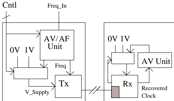
Fig. 3. Block Diagram of a Link
