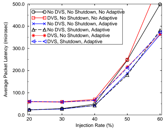
(b) Average Packet Latency
