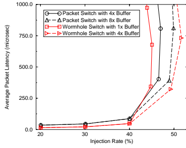
(a) Average Packet Latency
