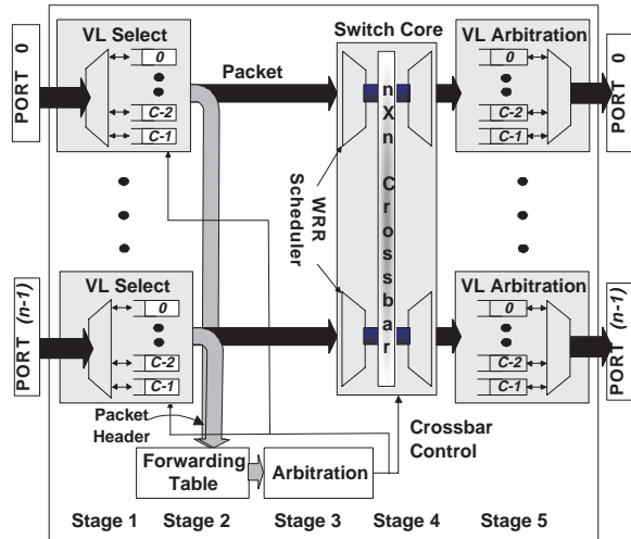
Fig. 1. A Pipelined Switch Architecture
