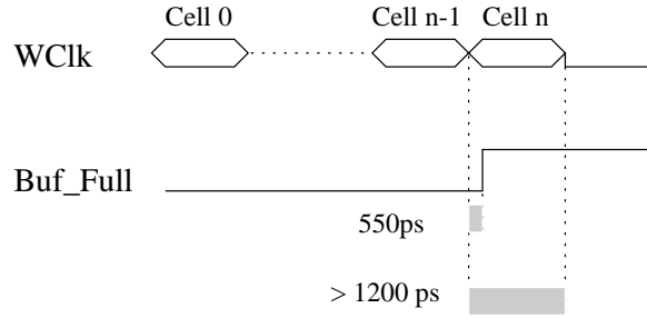
Fig. 5. Timing Diagram of Filling Buffer
