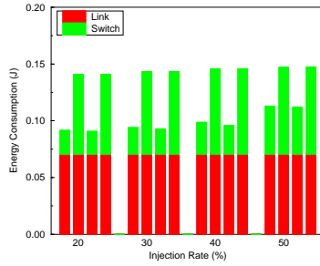
(c) Energy Distribution
