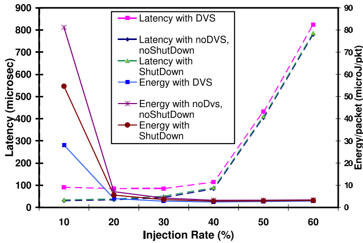
(a) Average Packet Latency
