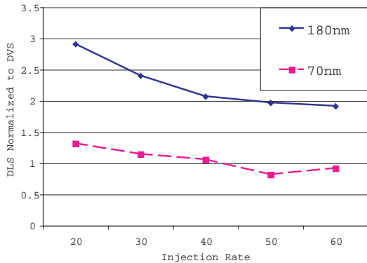
Fig. 11. Impact of Leakage Energy
