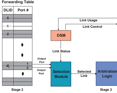
Fig. 6. Dynamic Shutdown Mechanism
