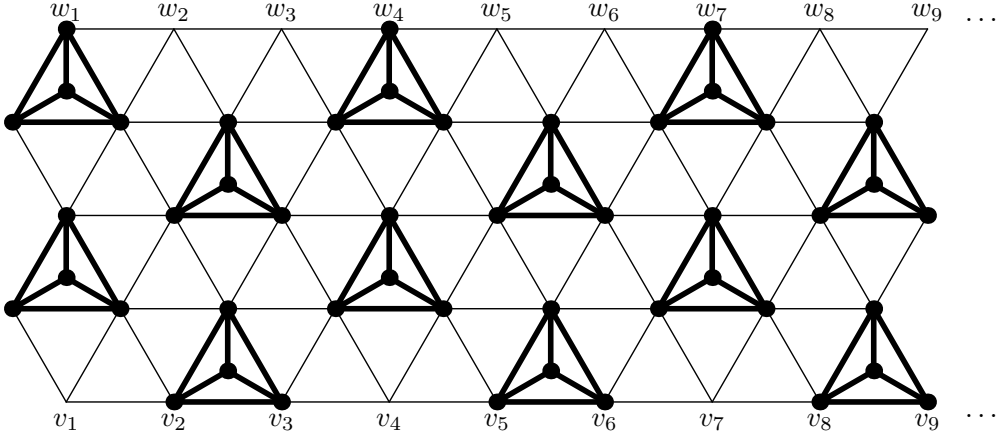
Figure 1: Building T_k : arranging k copies of K_4 in 4 layers of triangles.
