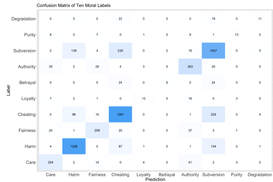
Figure 5: Confusion matrix of ten moral labels
