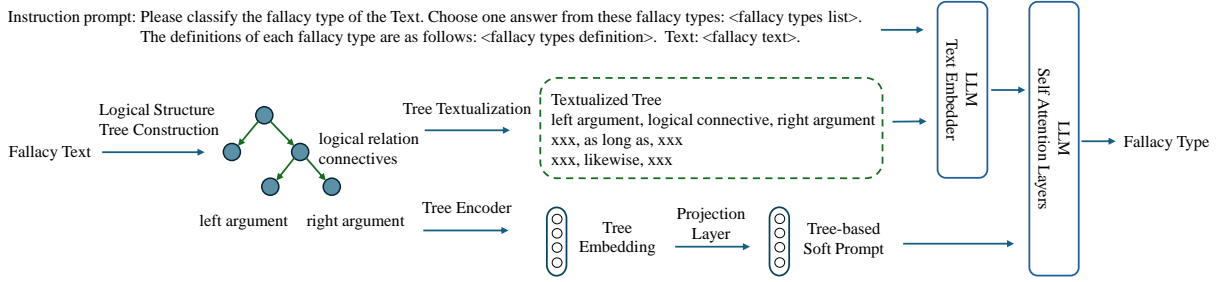
Figure 2: An illustration of logical fallacy classification informed by logical structure tree.
