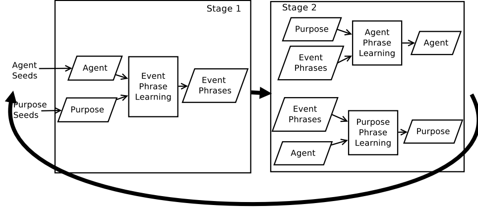
Figure 1.3. Bootstrapped Learning of Event Dictionaries, illustrated with Agents and Purpose as Event Facets.
