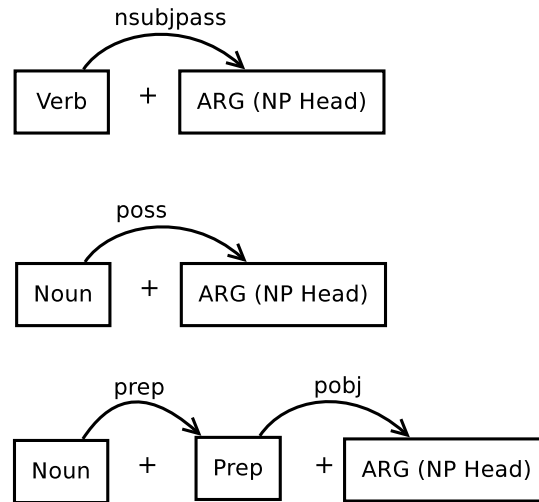
Figure 5.5. Three New Syntactic Structures to Extract Effect Phrases and Patient Terms for Terrorism Events
