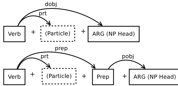
Figure 5.2. Phrasal Forms of Event & Purpose Phrases for Civil Unrest Events
