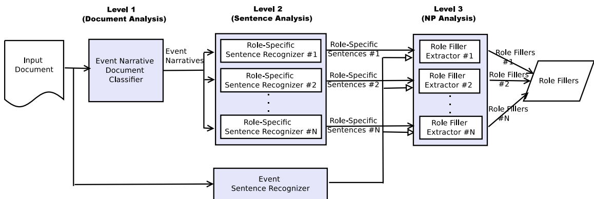
Figure 1.1. TIER: A Multi-Layered Architecture for Event Extraction
