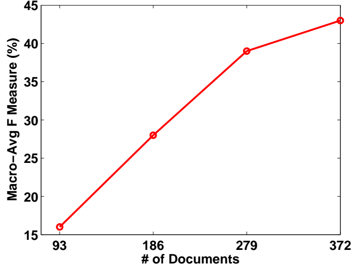
Figure 3.9. Learning Curve for TIER
