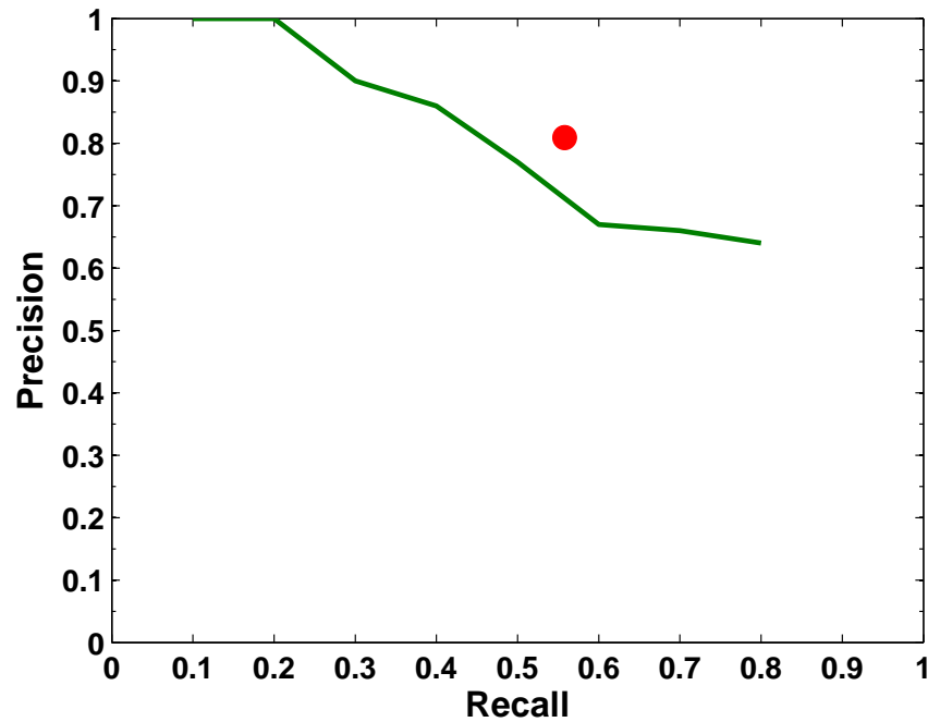
Figure 5.8. Comparison with the Terrier IR system, Terrorism Events
