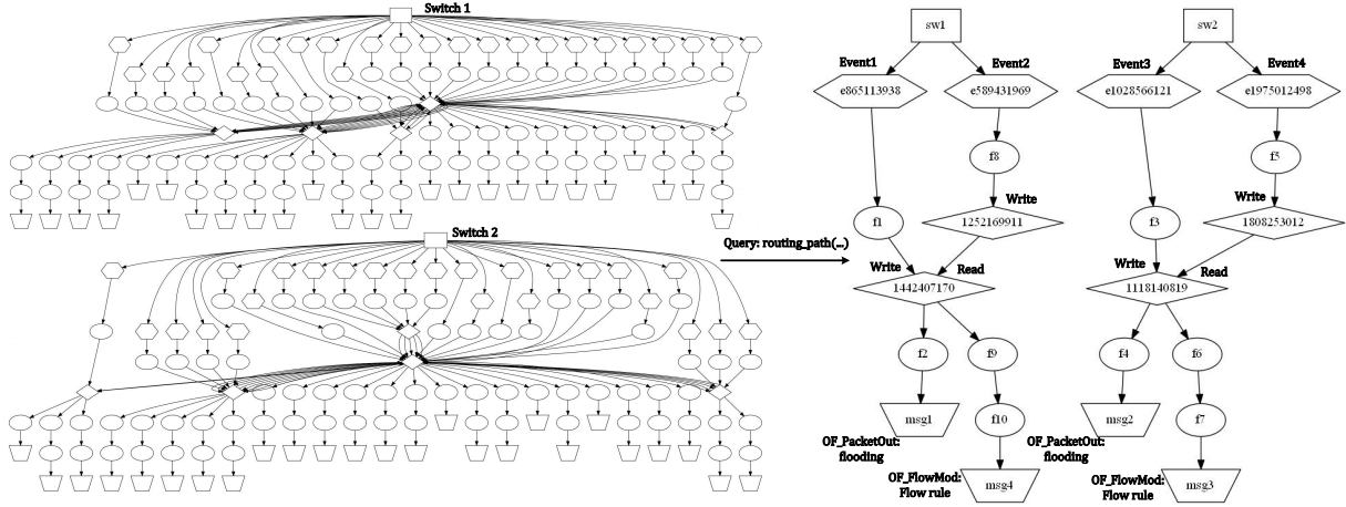
Figure 7: Simplified Dependency Graph of Execution Traces of the Running Example. Box denotes switches, Hexagon denotes events, Circle denotes function calls, Diamond denotes variable fields, Trapezium denotes OpenFlow messages.
