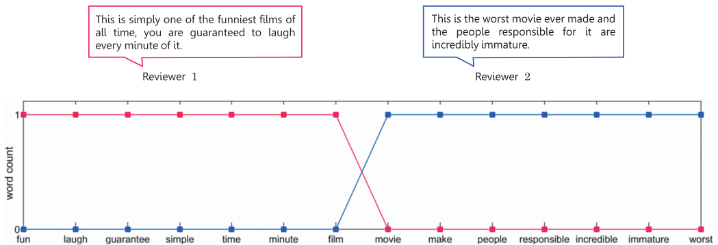
Fig. 4.23 BoW representation of two movie review excerpts, with words (after the removal of stop words and stemming) shared between the two reviews listed along the horizontal axis. The vastly different opinion of each review is reflected very well by the BoW histograms, which have zero correlation.
