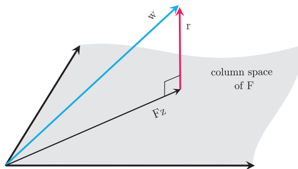
Fig. 7.1 An illustration of the fundamental theorem of linear algebra which states that any vector \mathbf{w} in an M -dimensional space can be decomposed as \mathbf{w} = \mathbf{Fz} + \mathbf{r} . Here the vector \mathbf{Fz} belongs in the subspace determined by the columns of the matrix \mathbf{F} and \mathbf{r} is orthogonal to this subspace.
