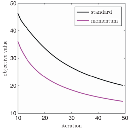
Fig. 7.6 The cost function value of the first k = 10 –50 iterations of standard and momentum gradient descent procedures (shown in black and magenta respectively) on a classification dataset, averaged over five runs. By tuning the momentum parameter we can create faster converging gradient descent schemes. See text for further details.
