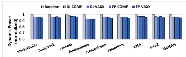
Figure 15: Dynamic Power Consumption Normalized to Baseline.
