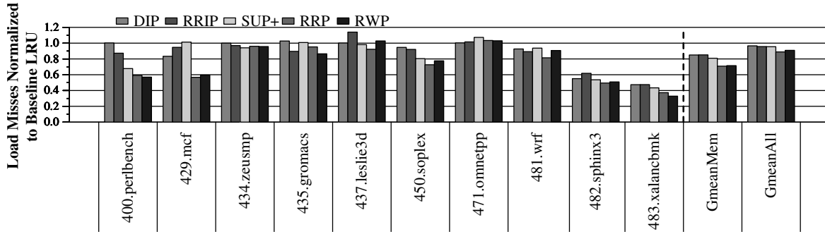
Figure 8: Normalized load miss count over baseline LRU.
