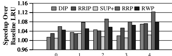
Figure 13: Normalized weighted speedup over LRU when the number of memory-intensive applications in a multi-programmed workload mix is varied.
