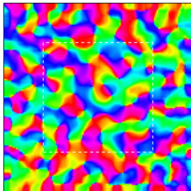
(b) Iteration 2000
