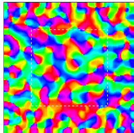
(c) Iteration 5000
