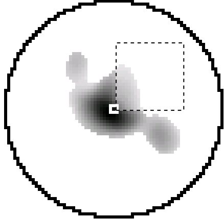
(b) Iteration 5000
