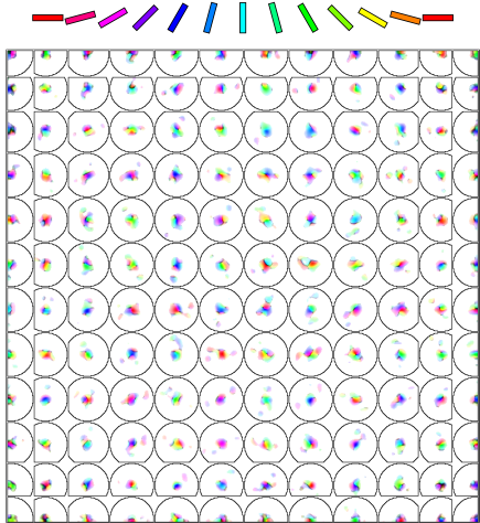
(b) Lateral inhibitory
