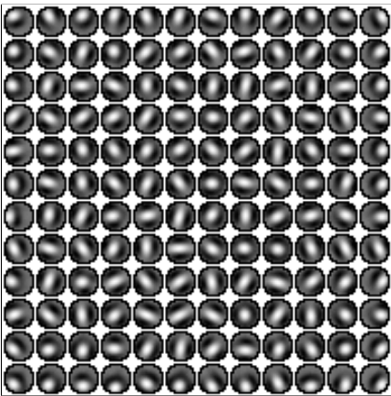
(a) Afferent (ON-OFF)
