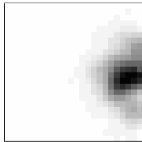
(c) Iteration 5000
