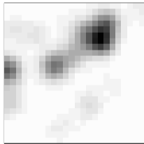
(b) Iteration 1000
