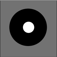
(a) ON cell in retina or LGN
