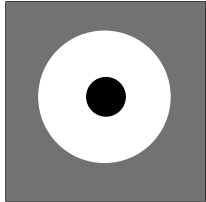
(b) OFF cell in retina or LGN
