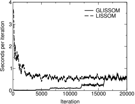
(a) Training time per iteration
