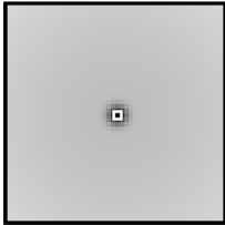
(b) Sum of Gaussians; isotropic
