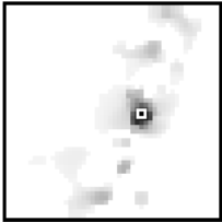
(a) Self-organized; 60^\circ preference
