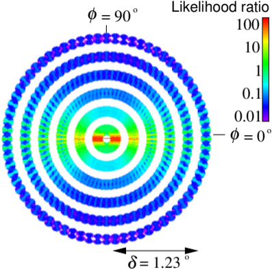
(a) Edge cooccurrence in nature
