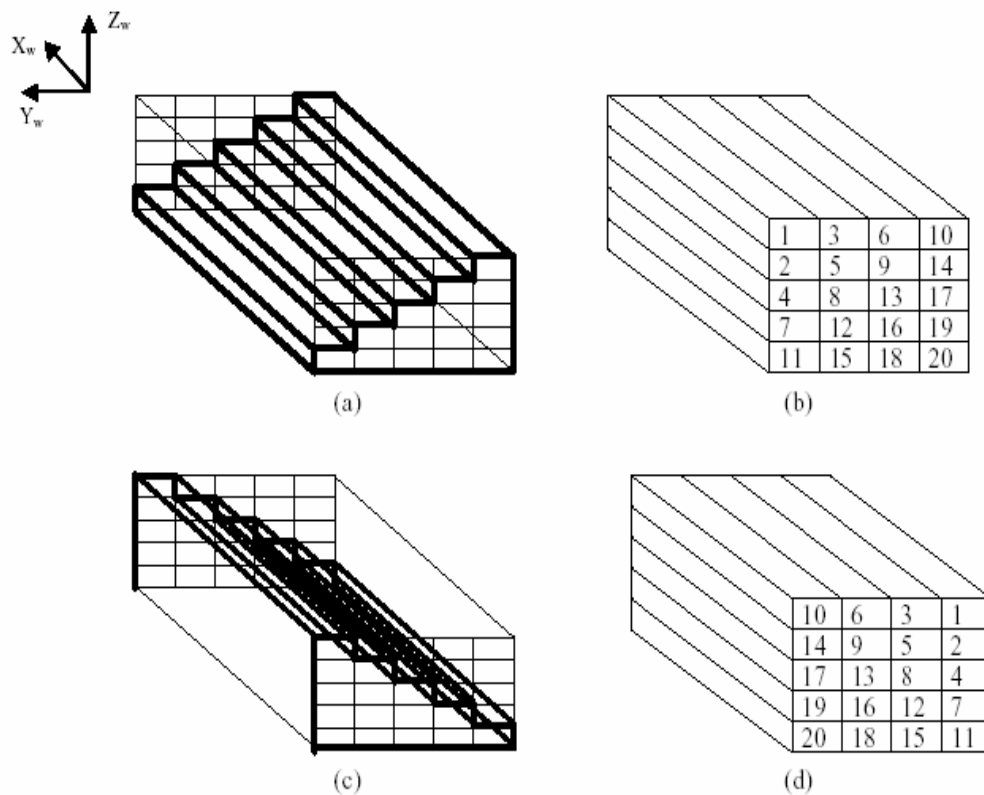
Fig. 2. Stair-step cutting.
