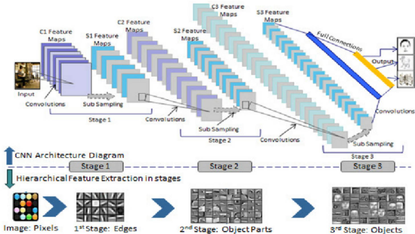
CNN Model
