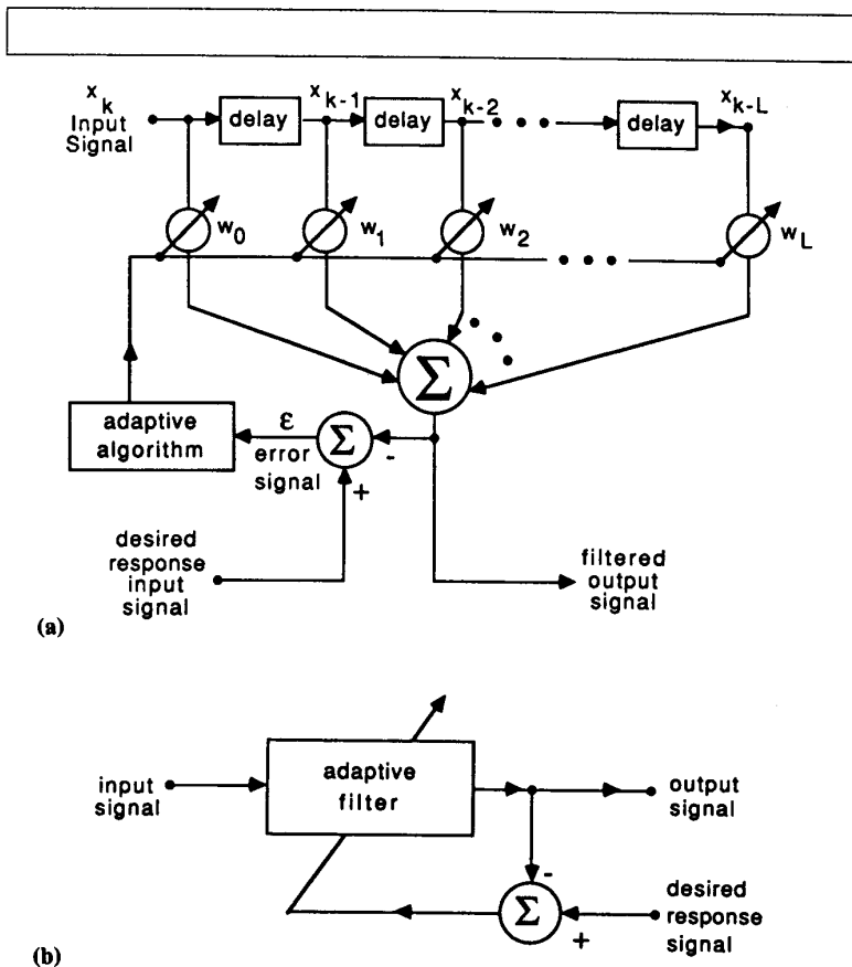
Figure 2. Adaptive digital filter: (a) details of a tapped-delay-line digital filter; (b) symbolic representation of an adaptive filter.
