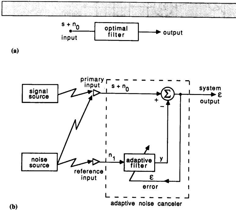
Figure 6. Separation of signal and noise: (a) classical approach; (b) adaptive noise-canceling approach.
